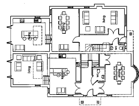
ground floor plans
